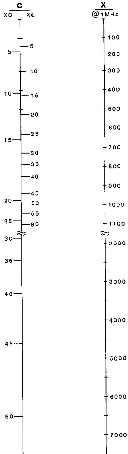
PICTORIAL 5-4
