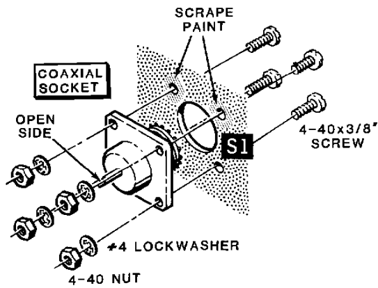
DETAIL 2-1A
