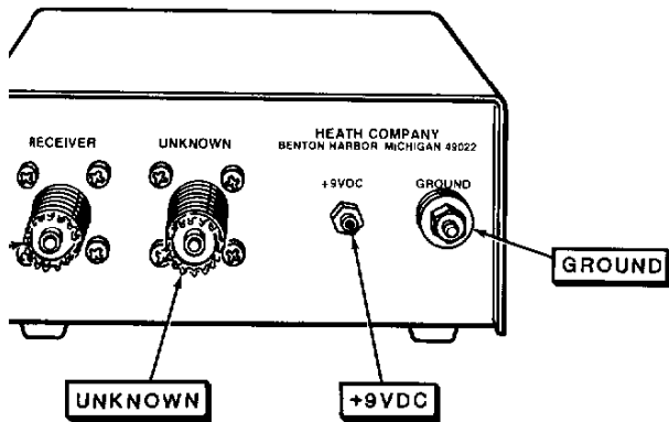
PICTORIAL 5-2
