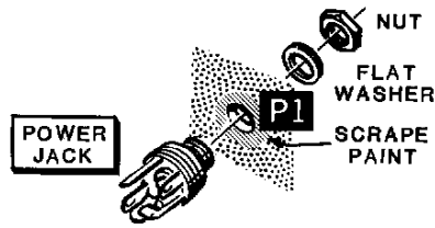
DETAIL 2-1B
