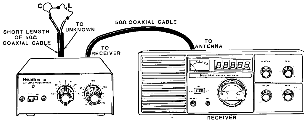
PICTORIAL 5-5
